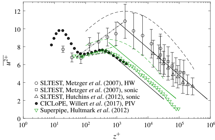
FIGURE 7. (Colour online) Comparison of \overline{u^{2+}} for the SLTEST surface layer (at Re_\tau \approx 10^6 ), Superpipe (at Re_\tau \approx 10^5 ) and CICLoPE pipe experiments (at Re_\tau \approx 40\,000 ) with the logarithmic model of (3.1) (—), the intermediate region correlation of (3.4) (- · -) and the curve fit proposed by Alfredsson et al. (2011) (---). The curve fit proposed by Alfredsson et al. (2011) is shown for Re_\tau = 10^5 and 10^6 .
