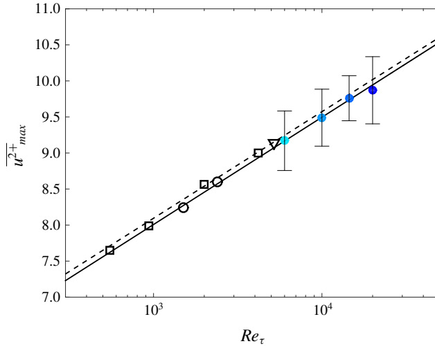
FIGURE 3. (Colour online) Dependence of maximum of \overline{u^{2+}} on Re_\tau . ●, NSTAP; ○, DNS of turbulent boundary layer from Sillero et al. (2013); □, DNS of channel flow from Lozano-Durán & Jiménez (2014); ▽, DNS of channel flow from Lee & Moser (2015); —, \overline{u^{2+}}_{max} = 3.54 + 0.646 \log(Re_\tau) ; - - -, \overline{u^{2+}}_{max} = 3.66 + 0.642 \log(Re_\tau) from Lee & Moser (2015).
